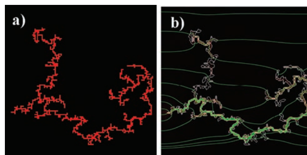
Figure 3. (a) Cluster structure from Monte Carlo simulation and (b) current density from subsequent FEM calculation. (c) Relative increase in conductivity for the formed structures during aggregation in comparison with the initial state at t = 0 . The final \sigma/\sigma_0 ratio was 2.1.
