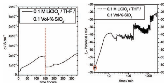
Figure 2. a. Time dependent conductivity in 0.1 M LiClO 4 /THF ( \phi(\text{SiO}_2) = 0.1\% ) in combination with ultrasonic treatment (pulses of low intensity with frequency of 0.2 Hz for 1 min) in between (dashed line). b. Time dependent \zeta -potential of 0.1 M LiClO 4 /THF/SiO 2 ( \phi(\text{SiO}_2) = 0.1\% ). A logarithmic scale on the time axis is used to highlight the initial value of the effective \zeta -potential.
